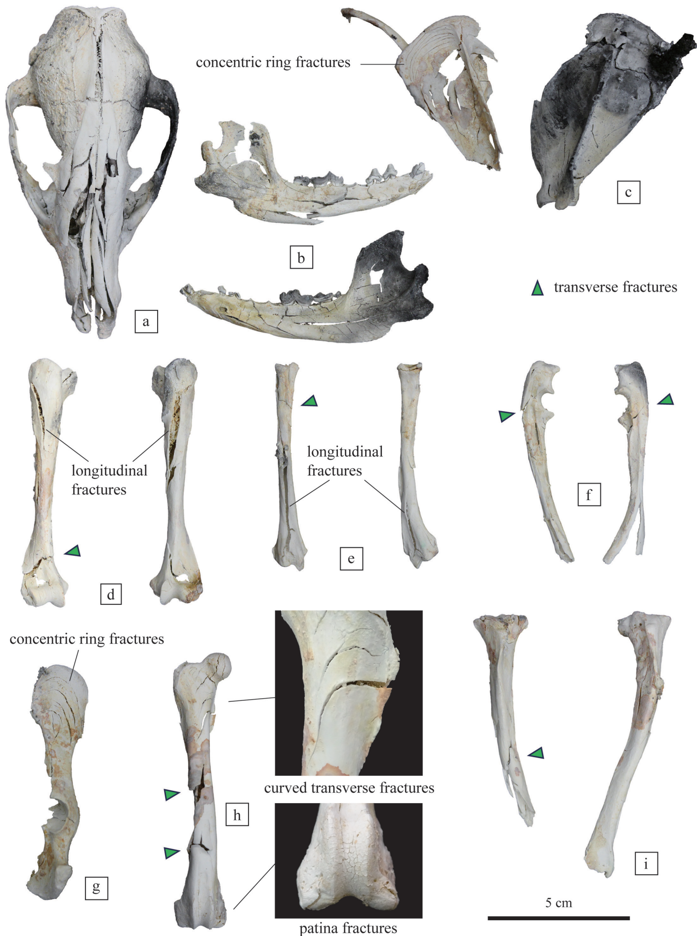
APPENDIX 3. DISCOLOURATION, DEFORMATION AND FRACTURES (RACCOON DOG: SAMPLE 3) (A) CRANIUM, (B) MANDIBLE, (C) SCAPULA, (D) HUMERUS, (E) RADIUS, (F) ULNA, (G) HIP BONE, (H) FEMUR, (I) TIBIA. THE CRANIUM, MANDIBLE AND SCAPULA EXHIBIT CLEAR LATERAL DIFFERENCES IN DISCOLOURATION, WITH GREATER DEFORMATION ON THE FLAME-EXPOSED RIGHT SIDE. PHOTOGRAPHS BY YASUSHI FURUSAWA.
